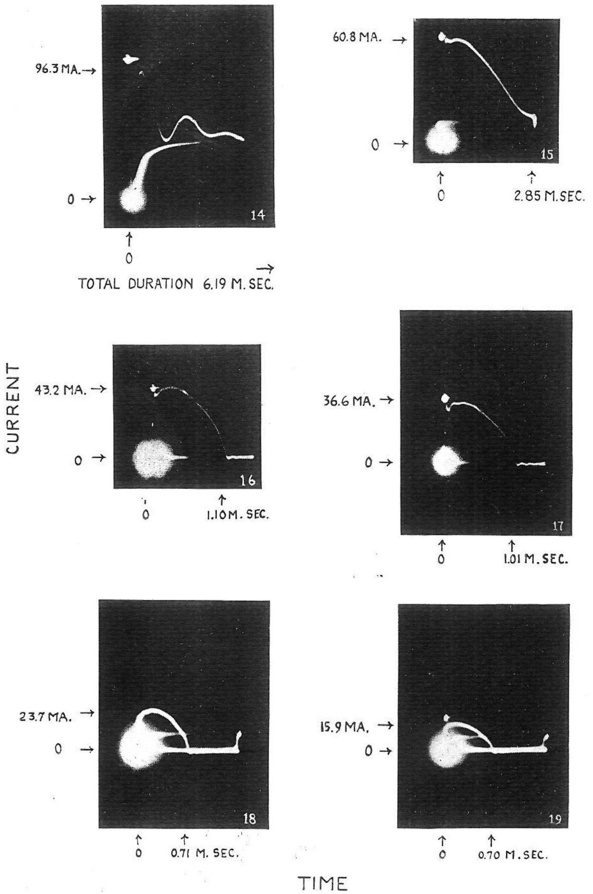
FIGS. 14-19. Oscillograph records of induction coil spark discharges
